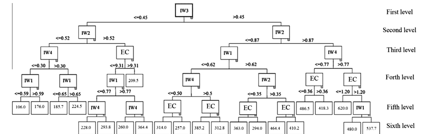
Fig. 1. Schematic structure of the derived DT- PF applied to spring wheat. EC: irrigation water salinity (dS m -1 ); IW1, IW2, IW3, IW4: relative irrigation water requirement at different growth stages (Table 2). The values inside the leaves are the predicted GY (g m -2 ).
